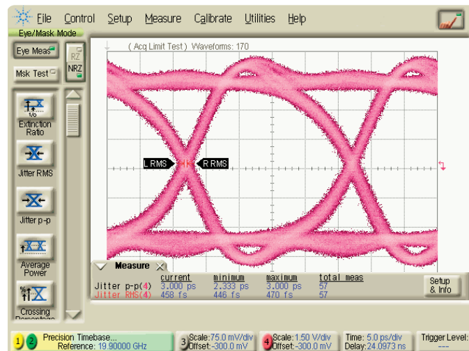
OPT003 (2 31 - 1) EYE: <500 fs added rms jitter (5 ps/div)
