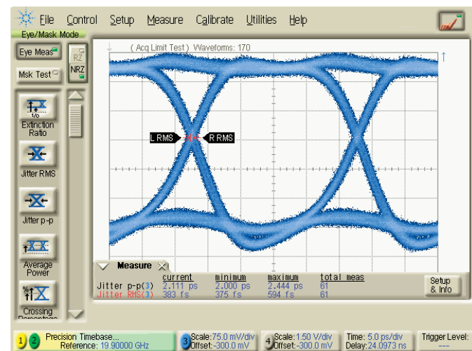
OPT003 (2 31 - 1) EYE: Input signal from PRBS Generator
